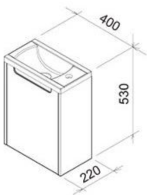
SD Classic 400 + Classic 400
